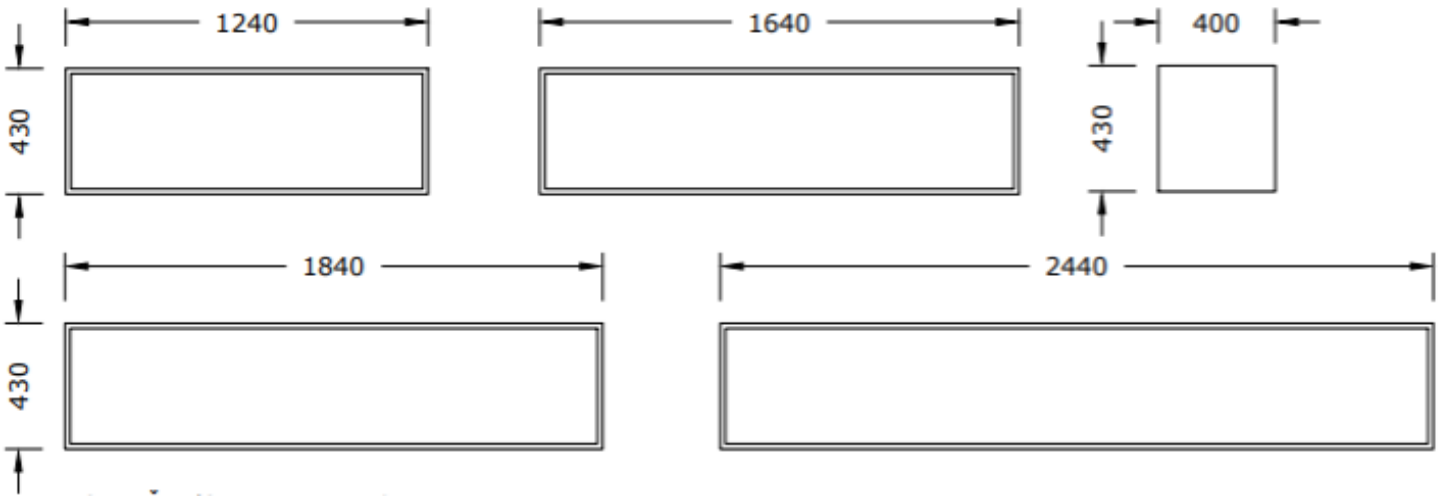
DRAWER / CABINET
