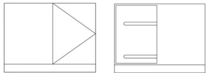
WITH SINGLE DOOR AND CORNER SYSTEM / WIDTH: 450;500;600 mm
